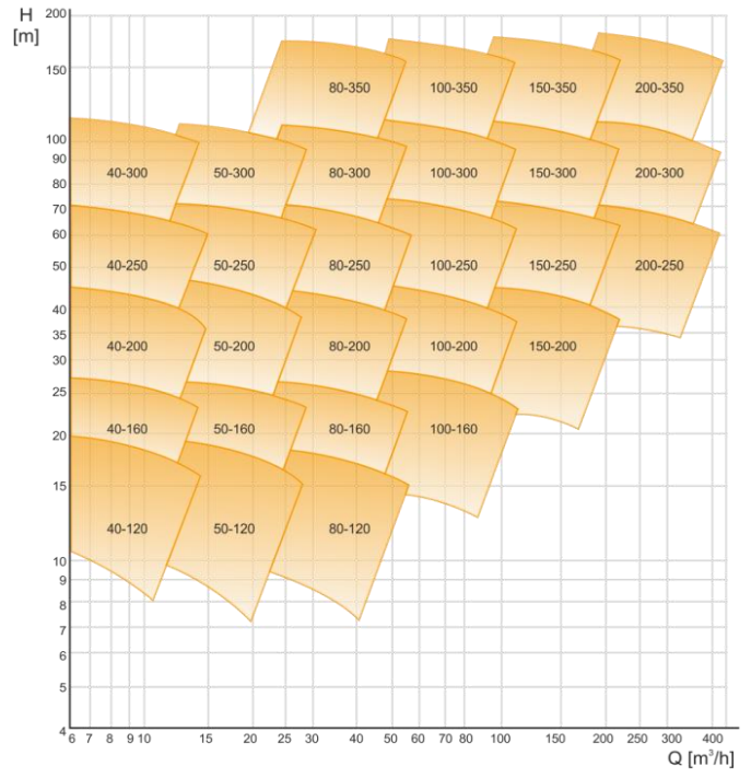
50Hz 3000 RPM
