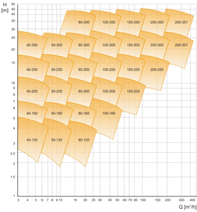
50Hz 1500 RPM
